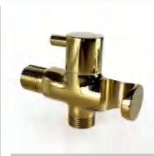
GZXF288255G $4.00 Weight: 240g Material: Brass Single package size: 108*60*55mm Outer box size: 560*295*405mm Quantity / box: 200 pieces
