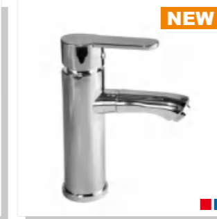
GZCPS015020-1 $3.30 Description: Chrome Rotate Mixer Basin Faucet Weight: 670g Material: Zinc alloy Single package size: 250*190*70mm Outer box size: 520*390*440mm Quantity / Ctn: 24 pieces
