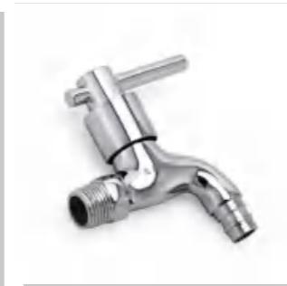
GZSH110768558 $1.53 Weight: 165g Material: Brass Single package size: 124*108*30mm Outer box size: 640*330*450mm Quantity / box: 200 pieces
