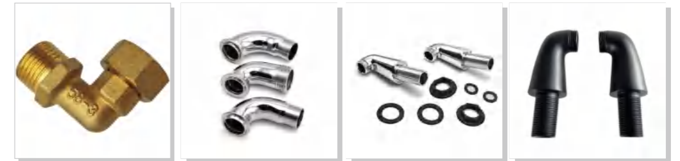
GZHMB77040 $0.95 GZHY0085535 $1.74 GZ236012 $2.20 GZ236012B $2.50 Weight: 77g Material: Brass Single package size: NONE Outer box size: 560*295*405mm Quantity / box: 500 pieces Weight: 72-95g Material: Brass Single package size: Outer box size: 640*330*450mm Quantity / box: 200 pieces Weight: 230g Material: Zinc alloy Single package size: 160*100*30mm Outer box size: 560*290*410mm Quantity / box: 100 pieces Weight: 230g Material: Zinc alloy Single package size: 160*100*30mm Outer box size: 560*290*410mm Quantity / box: 100 pieces
