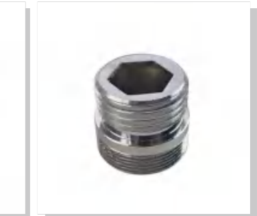
GZHMB29020 $0.39 Weight: 14g Material: Brass Single package size: NONE Outer box size: 560*295*405mm Quantity / box: 500 pieces
