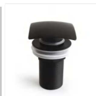
GZDTFS328018B $3.80 Function: Black Bounce Sewer Weight: 280g Material: Stainless steel Product size: 110*75*75mm Outer Ctn size: 560*390*320mm Quantity / Ctn: 100 pieces
