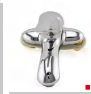
GZ0016 $4.25 Weight: 475g Material: Zinc alloy Single package size: 200*160*140mm Outer box size: 620*340*440mm Quantity / box: 18 pieces
