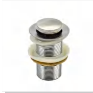
GZ0168DTF95 $2.10 Function: Basin Drainer Weight: 165g Material: Stainless steel Product size: 110*75*75mm Outer Ctn size: 560*290*350mm Quantity / Ctn: 100 pieces
