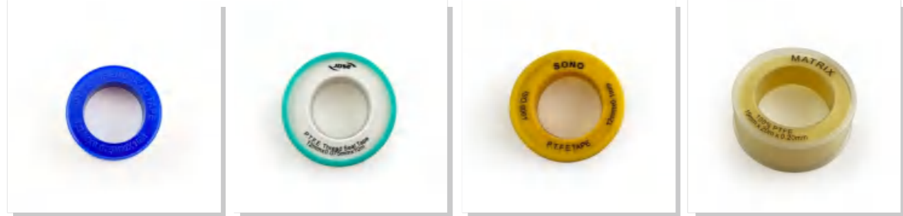
GZTW403002024 $0.047 GZTWP563010029 $0.063 GZTW563302025 $0.042 GZTWP613515038 $0.08 Weight: 5g Material: P.T.F.E Tape size: 12mm*0.075mmx10m Outer box size: 440*440*260mm Quantity / box: 500 pieces Weight: 8g Material: P.T.F.E Tape size: 19mm*0.2mmx10m Outer box size: 440*440*260mm Quantity / box: 500 pieces Weight: 7g Material: P.T.F.E Tape size: 12mm*0.1mmx10m Outer box size: 440*440*260mm Quantity / box: 500 pieces Weight: 10g Material: P.T.F.E Tape size: 19mm*0.2mmx15m Outer box size: 440*440*260mm Quantity / box: 500 pieces
