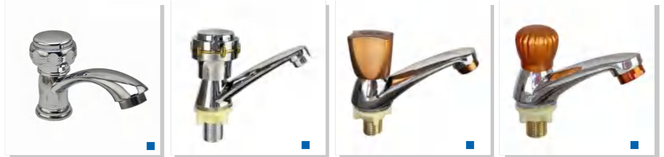
GZAY055 $1.95 Weight: 215g Material: Zinc alloy Single package size: 200*160*140mm Outer box size: 620*340*440mm Quantity / box: 144 pieces GZ7S1574008 $1.50 Weight: 230g Material: Zinc alloy Single package size: 200*160*80mm Outer box size: 620*340*440mm Quantity / box: 120 pieces GZD99XX086ZX076-1 $2.55 Weight: 305g Material: Zinc alloy Single package size: 200*160*80mm Outer box size: 620*340*440mm Quantity / box: 120 pieces GZD99XX086ZX076-2 $2.55 Weight: 300g Material: Zinc alloy Single package size: 200*160*80mm Outer box size: 620*340*440mm Quantity / box: 120 pieces
