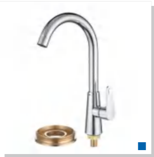
GZBS420025 $4.80 Weight: 420g Material: Zinc alloy Single package size: 370*215*70mm Outer box size: 660*380*450mm Quantity / box: 54 pieces
