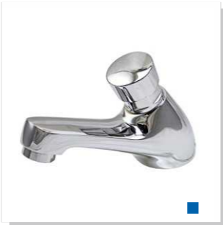
GZBHY518036 $7.10 Weight: 520g Material: Brass Single package size: 162*125*52mm Outer box size: 560*290*410mm Quantity / box: 60 pieces
