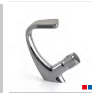
GZHLB698075 $18.00 Description: Kitchen Faucet Pipe Weight: 445g Material: PP+SS Single package size: 330*170*75mm Outer box size: 700*340*400mm Quantity / Ctn: 60 pieces
